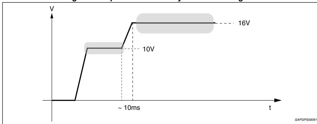
Figure 36. Upwards fast battery transitions diagram
